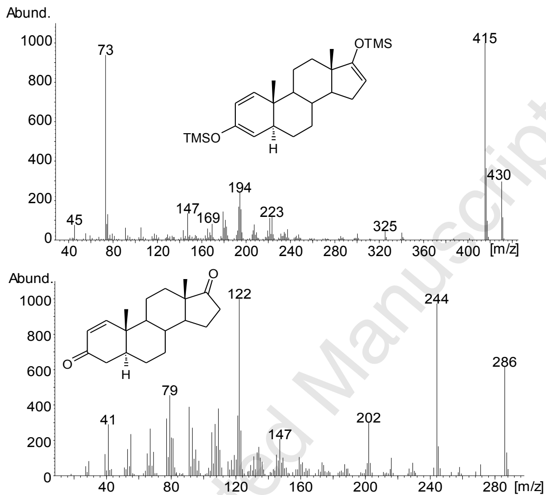
figure 2: Mass spectra of 5 \alpha -androst-1-ene-3,17-dione (2), upper bis-TMS, M^+ = 430 , lower underivatized, M^+ = 286
