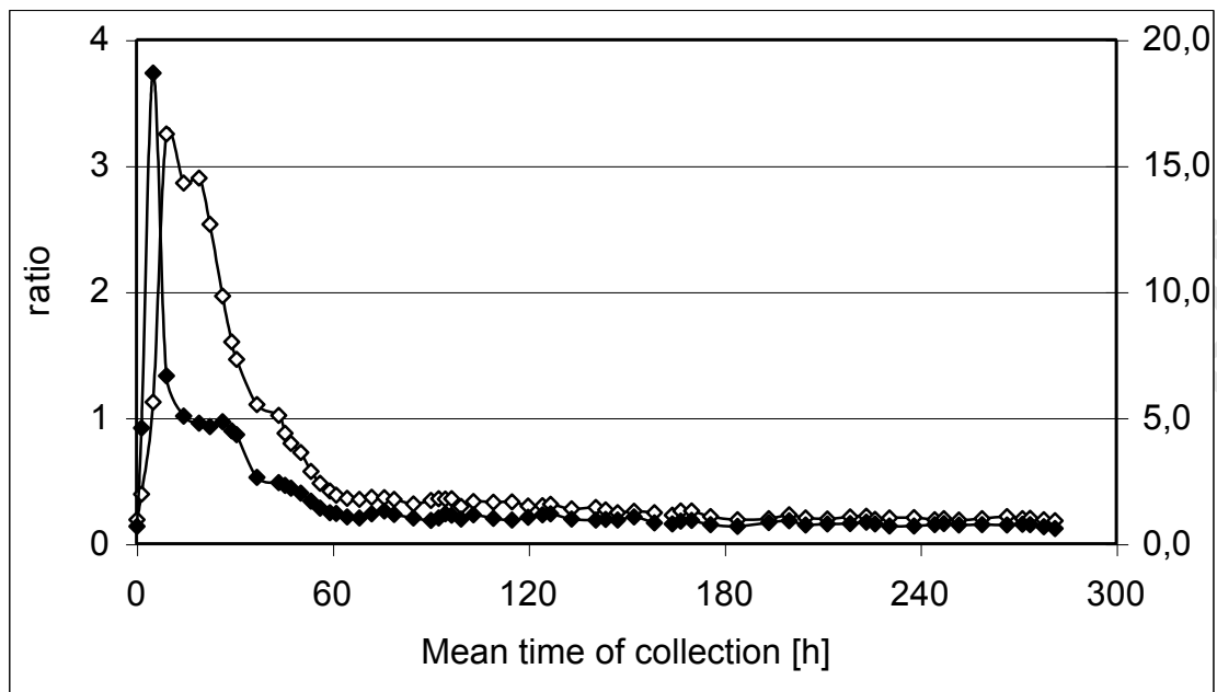
figure 12: Time course of AND/ETIO (◆, right y-axis) and Adiol/Bdiol ratio (◇, left y-axis) after oral administration of one capsule of “1-Androsterone”, data shown using midpoints of collection periods
