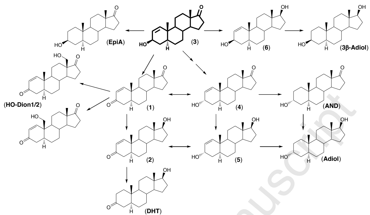
Proposed metabolism of 3β-hydroxy-5α-androst-1-en-17-one (3)
