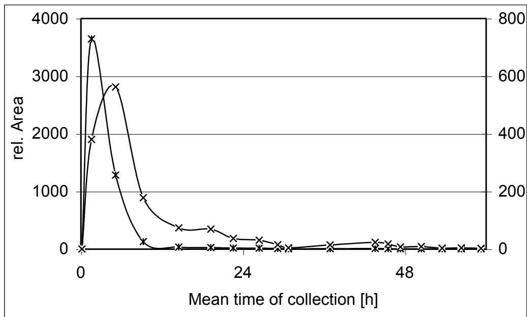
figure 11: Elimination kinetics of HO-Dione1 (*, left y-axis) and HO-Dione2 (x, right y-axis) after one capsule of "1-Androsterone", data shown using midpoints of collection periods and concentrations in 1000 fold peak area of analyte divided by area of internal standard
