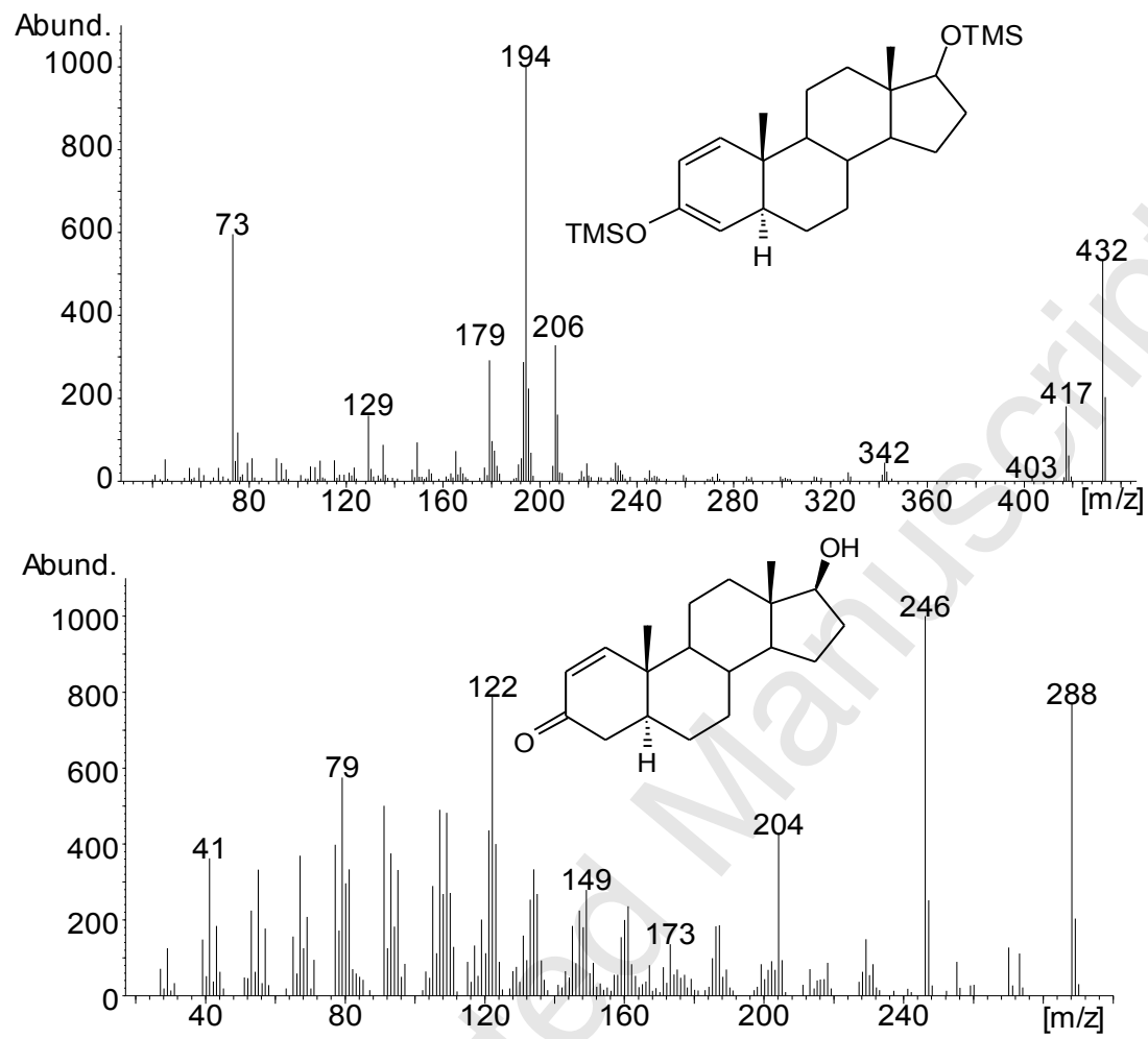
figure 1: Mass spectra of 17β-hydroxy-5α-androst-1-en-3-one (1-testosterone, (1)), upper bis-TMS, M^+ = 432 , lower underivatized, M^+ = 288
