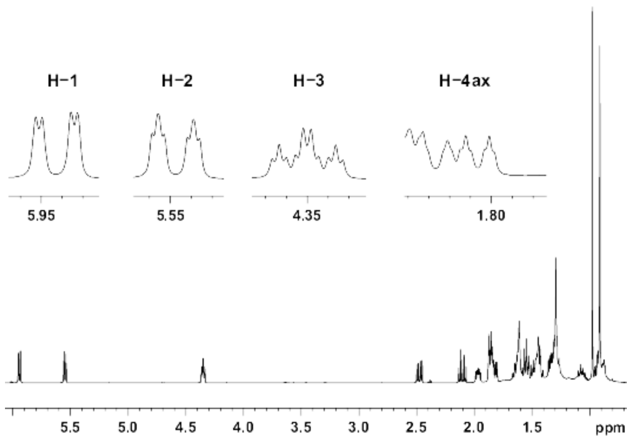
figure 6: 1 H-NMR spectrum (500 MHz, CDCl 3 , 298 K) of 3β-hydroxy-5α-androst-1-en-17-one (3), extracted from the product "1-Androsterone"
