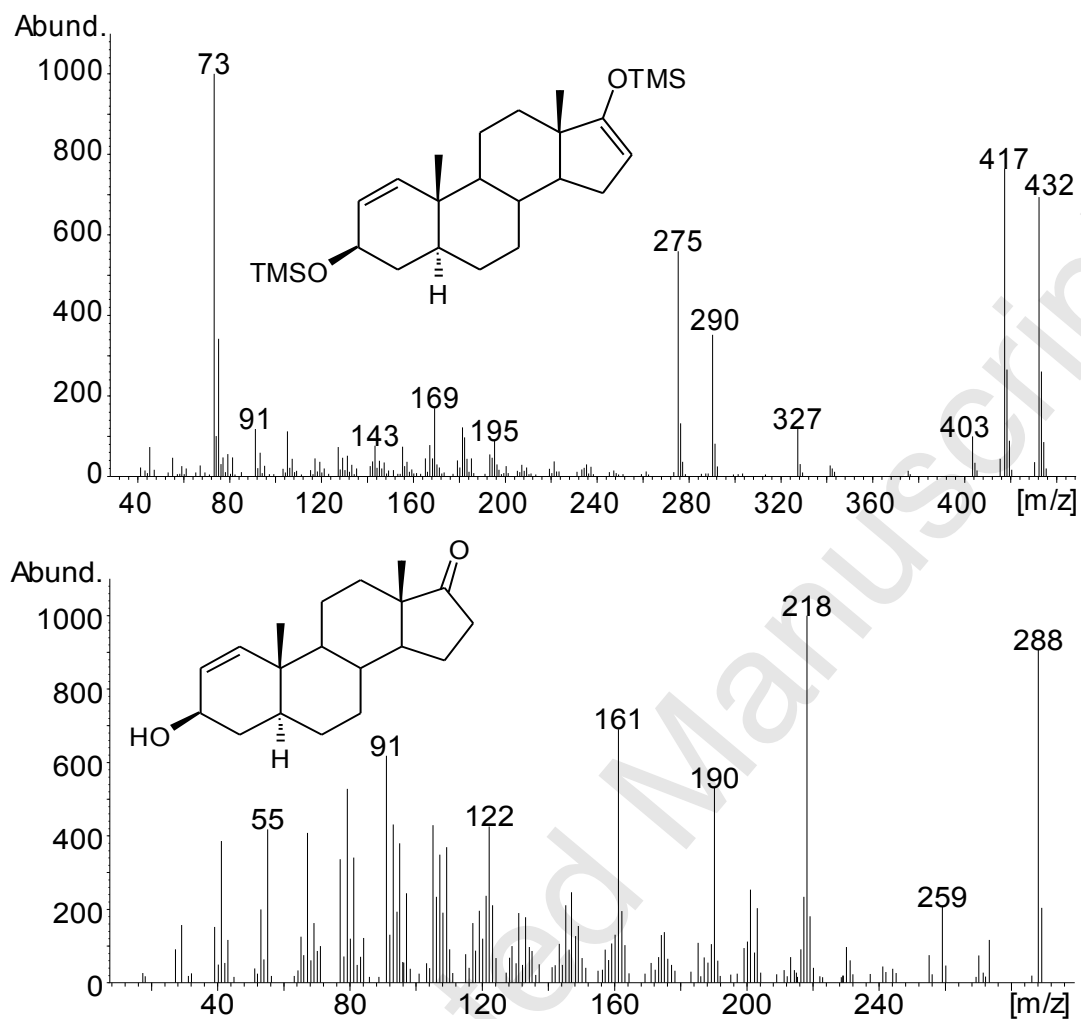
figure 3: Mass spectra of 3β-hydroxy-5α-androst-1-en-17-one (3), upper bis-TMS, M^+ = 432 , lower underivatized, M^+ = 288
