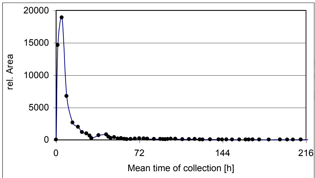
figure 9: Elimination kinetics of 3 \alpha -hydroxy-5 \alpha -androst-1-en-17-one (4, ●, main metabolite) after one capsule of “1-Androsterone”, data shown using midpoints of collection periods and concentrations in 1000 fold peak area of analyte divided by area of internal standard
