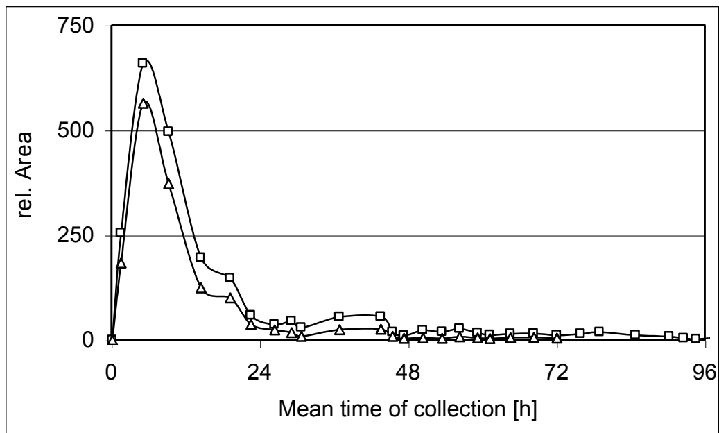
figure 10: Elimination kinetics of 5\alpha -androst-1-ene- 3\alpha,17\beta -diol (5, □) and 5\alpha -androst-1-ene- 3\beta,17\beta -diol (6, Δ) after one capsule of “1-Androsterone”, data shown using midpoints of collection periods and concentrations in 1000 fold peak area of analyte divided by area of internal standard
