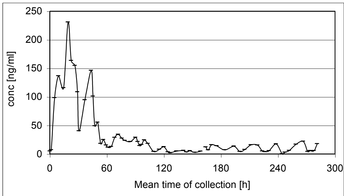
figure 13: Time course of EpiAND (—, concentrations not adjusted for density) after oral administration of one capsule of “1-Androsterone”, data shown using midpoints of collection periods
