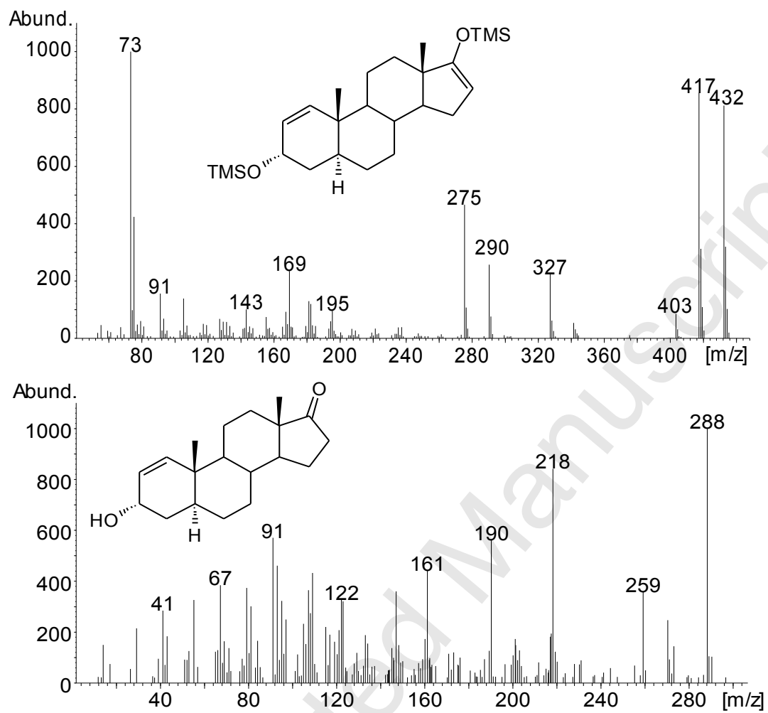
figure 4: Mass spectra of main metabolite, identified as 3α-hydroxy-5α-androst-1-en-17-one (4), upper bis-TMS, M^+ = 432 , lower underivatized, M^+ = 288
