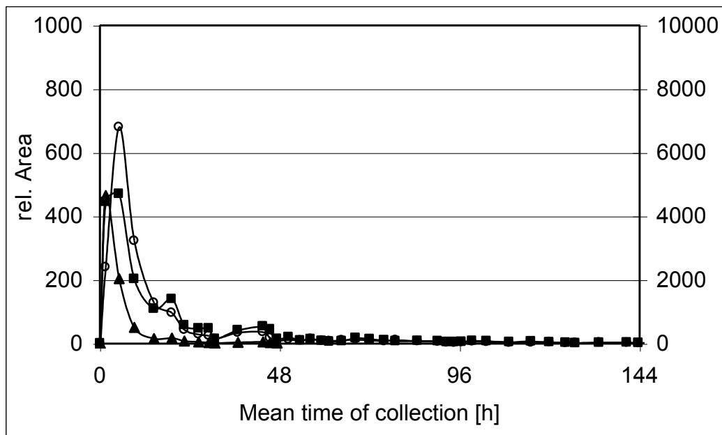
figure 8: Elimination kinetics of 3\beta -hydroxy- 5\alpha -androst-1-en-17-one (3, ▲ left y-axis), 17\beta -hydroxy- 5\alpha -androst-1-en-3-one (1, ○, right y-axis), and 5\alpha -androst-1-ene-3,17-dione (2, ■, left y-axis), after one capsule of “1-Androsterone”, data shown using midpoints of collection periods and concentrations in 1000 fold peak area of analyte relative to area of internal standard
