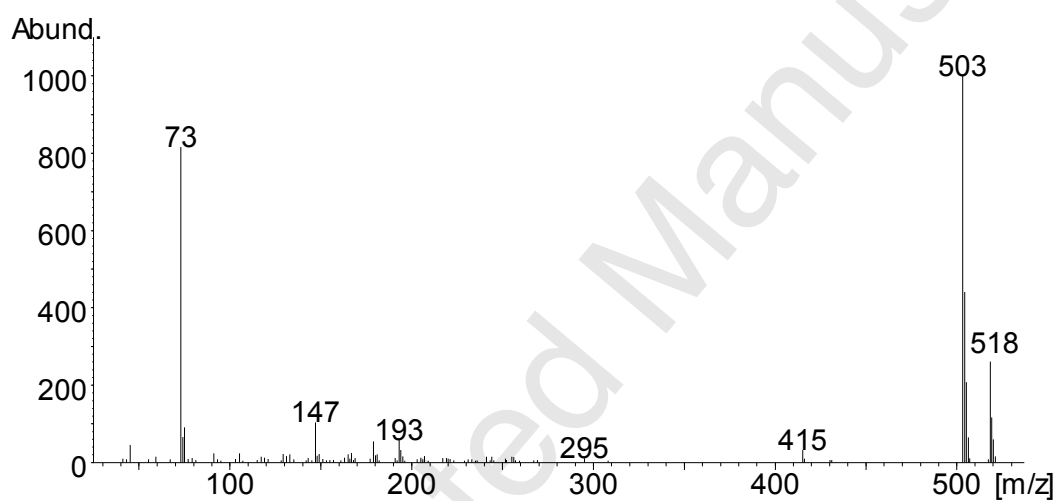
figure 7: Mass spectra of hydroxylated metabolites as tris-TMS derivatives upper: HO-Dione1 (M + = 518, RRT = 1.14), lower HO-Dione2 (M + = 518, RRT = 1.26)
